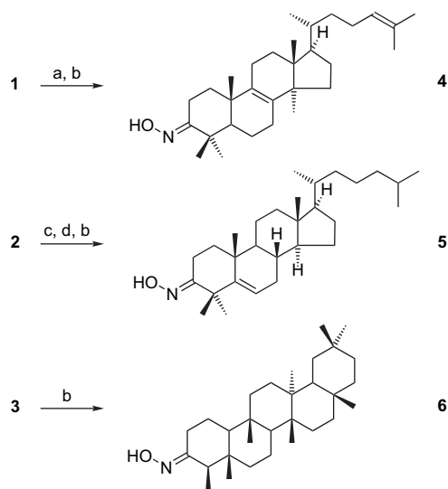
Scheme 1. (a) Jones' reagent, acetone, 0 °C to rt; (b) \text{NH}_2\text{OH}\cdot\text{HCl} , \text{NaHCO}_3 , EtOH, reflux; (c) \text{Br}_2 , AcOH, NaOAc, \text{Et}_2\text{O} , rt, \text{Na}_2\text{Cr}_2\text{O}_7\cdot 2\text{H}_2\text{O} , AcOH, 90 °C then Zn, AcOH, pyridine, rt; (d) K, ^t\text{BuOH} , MeI.
