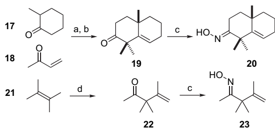
Scheme 4. (a) concd \text{H}_2\text{SO}_4 , reflux; (b) \text{KO}^t\text{Bu} , MeI, ^t\text{BuOH} , reflux; (c) \text{NH}_2\text{OH}\cdot\text{HCl} , \text{NaHCO}_3 , EtOH, reflux.
