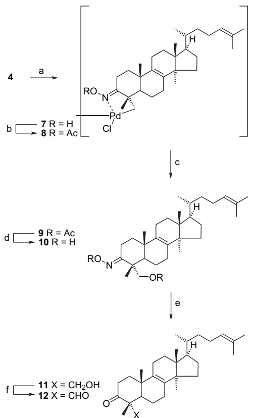
Scheme 2. (a) \text{Na}_2\text{PdCl}_4 , NaOAc, AcOH, rt, 88%; (b) \text{Ac}_2\text{O} , \text{Et}_3\text{N} , DMAP, \text{CH}_2\text{Cl}_2 , rt; (c) pyridine, \text{Pb}(\text{OAc})_4 , THF, AcOH then \text{NaBH}_4 , NaOH, 0 °C, 83% over two steps; (d) \text{Na}_2\text{CO}_3 , MeOH, rt, 95%; (e) \text{TiCl}_3 , HCl, \text{NH}_4\text{OAc} , \text{H}_2\text{O} , THF, rt, 85%; (f) \text{SO}_3\cdot\text{Py} , \text{Et}_3\text{N} , DMSO, rt, 52%.
