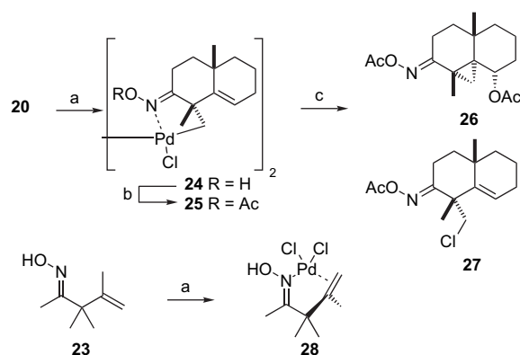
Scheme 5. (a) \text{Na}_2\text{PdCl}_4 , NaOAc, AcOH, rt, 85% ( 24 ), 52% ( 28 ); (b) \text{Ac}_2\text{O} , \text{Et}_3\text{N} , DMAP, \text{CH}_2\text{Cl}_2 , rt; (c) pyridine, \text{Pb}(\text{OAc})_4 , THF, AcOH then \text{NaBH}_4 , NaOH, 0 °C, 64% ( 26 ), 23% ( 27 ) over two steps.
