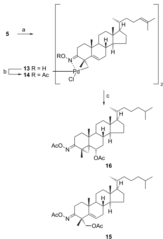
Scheme 3. (a) \text{Na}_2\text{PdCl}_4 , NaOAc, AcOH, rt, 91%; (b) \text{Ac}_2\text{O} , \text{Et}_3\text{N} , DMAP, \text{CH}_2\text{Cl}_2 , rt; (c) pyridine, \text{Pb}(\text{OAc})_4 , THF, AcOH then \text{NaBH}_4 , NaOH, 0 °C, 81% over two steps.
